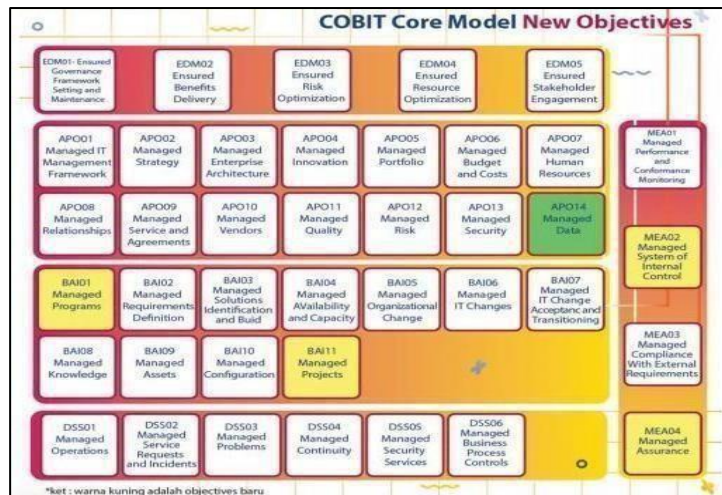
Gambar 4 Domain COBIT 2019
