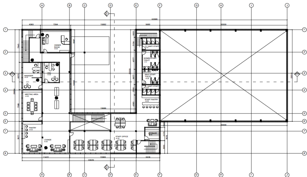
Gambar 4. 17 General layout lantai 2
